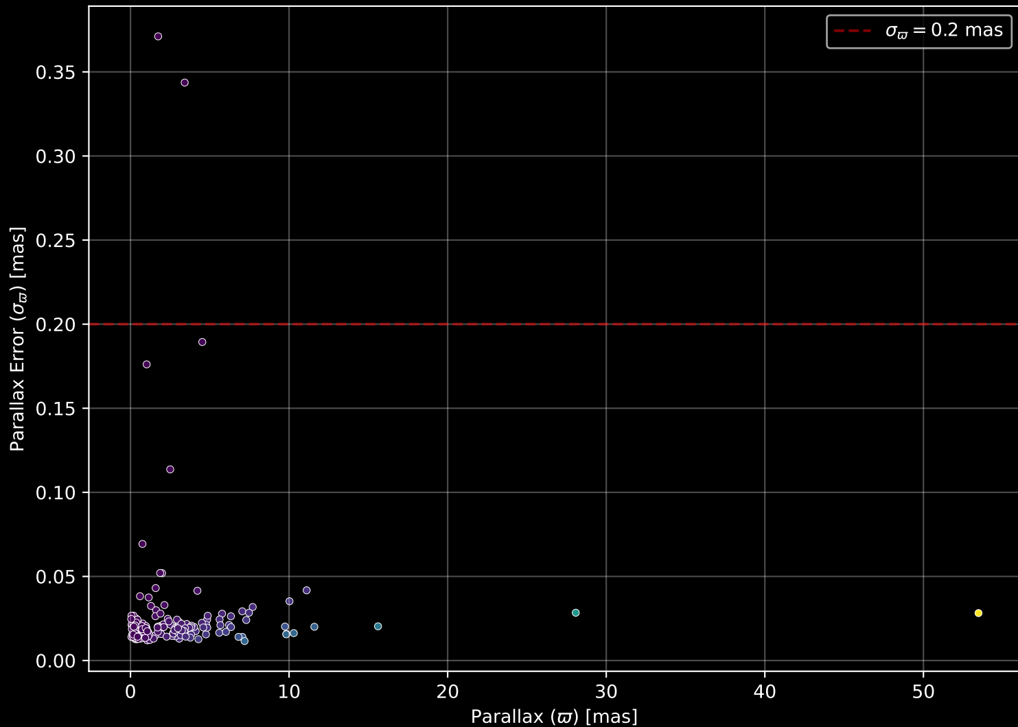
APOGEE DR17 Field: [020+60] Parallax Quality (n= 182)
