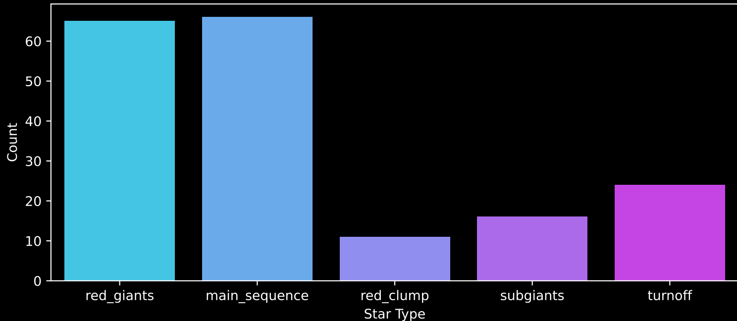
APOGEE DR17 Field: [020+60] Count plot of Star Type
