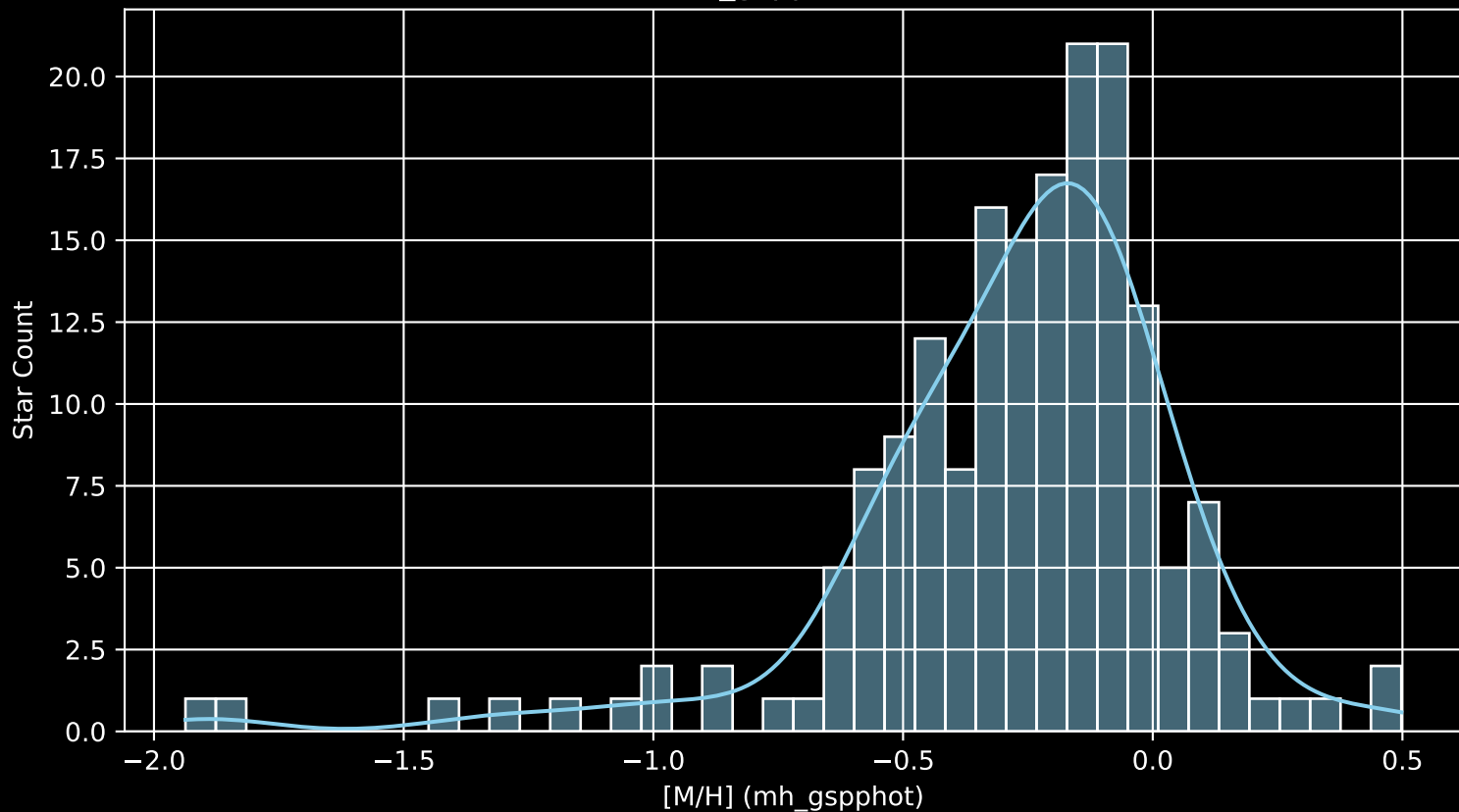
APOGEE DR17 Field: [020+60 [M/H] (mh_gspphot) (n= 177)
