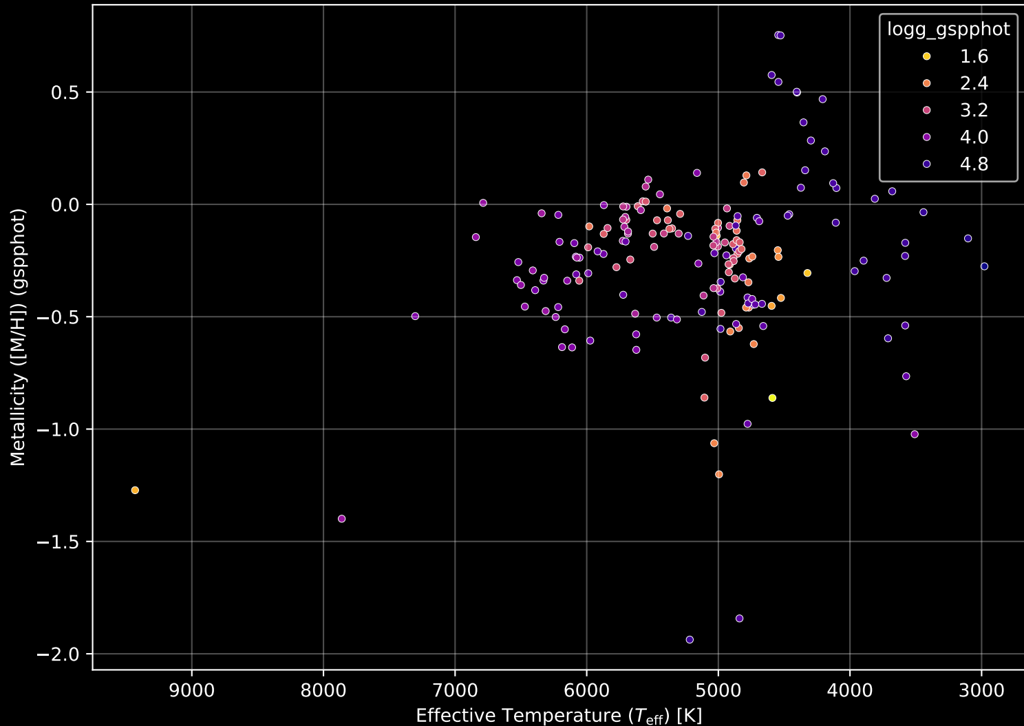
APOGEE DR17 Field: [020+60] Stellar Population Parameters (n= 182)
