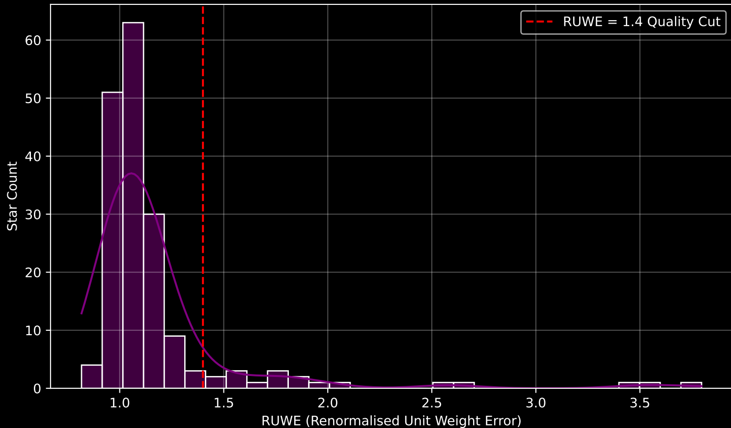
GAPOGEE DR17 Field [020+60] RUWE Distribution (n= 178)
