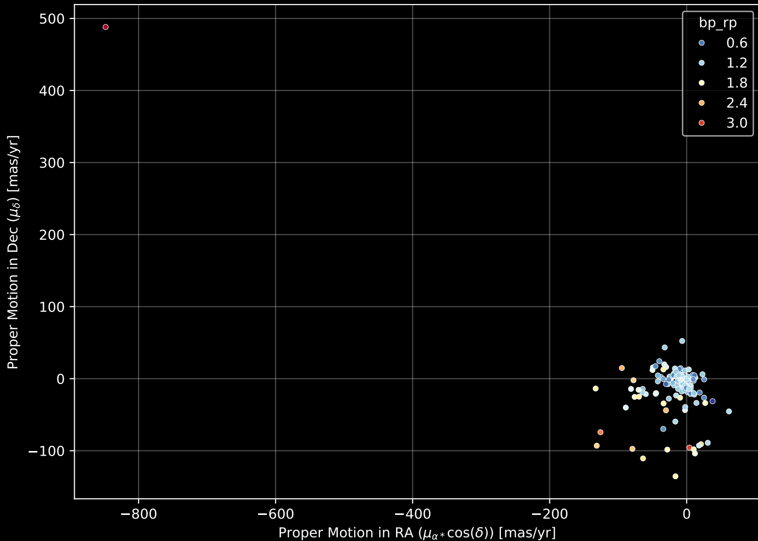
APOGEE DR17 Field: [020+60] Proper Motion Diagram (n= 182)
